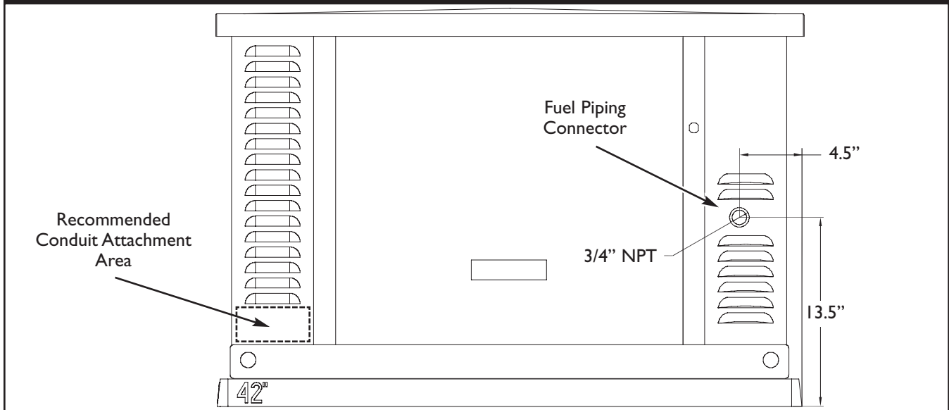
Figure 2 — Generator Fuel and Conduit Attachment Locations, Oil Service Side of Unit
